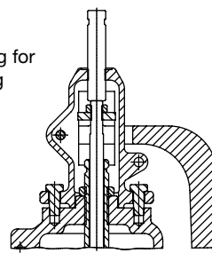
Open Lever (Single Acting Lever) 2600 Series, Types 26( )A10, A11, A20, A21, All Sizes Except 8x10
