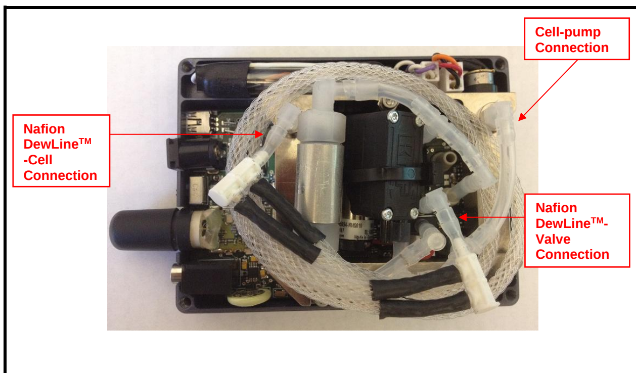
Figure 12.3. Inside View.
