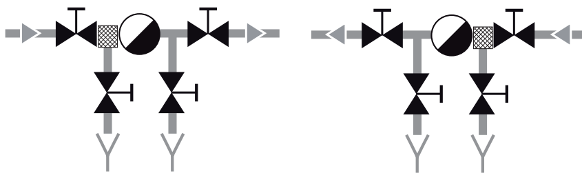
TS 36-1 Flow direction from left to right
