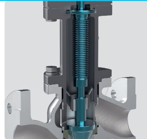
Bellows seal
