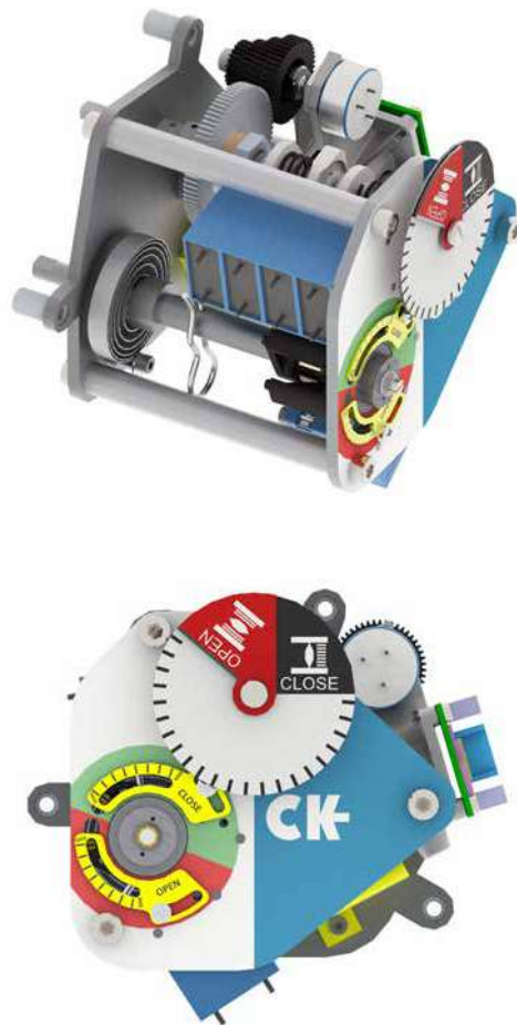
Part-turn CKQ Mechanical Switch Mechanism (MSM)
